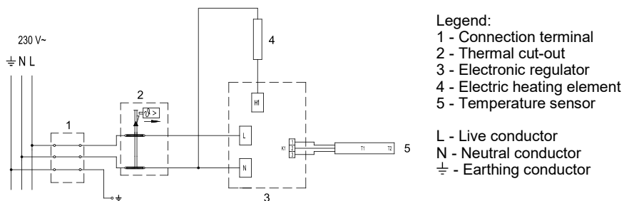
Fig. 5: Electric installation
