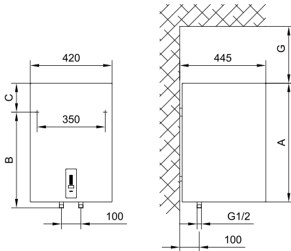
Fig. 1: Vertical installation on a wall
